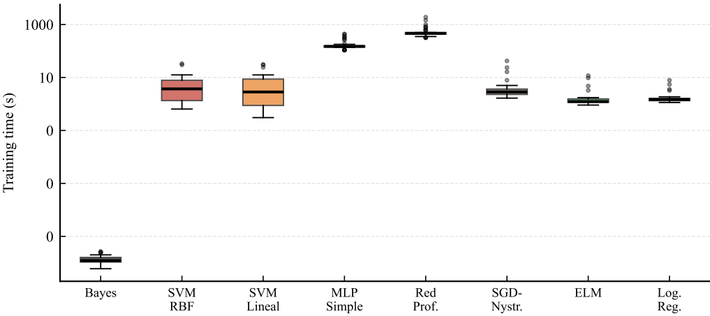
t_{train} distribution — E_b/N_0 \in [6, 8, 10, 12] dB
